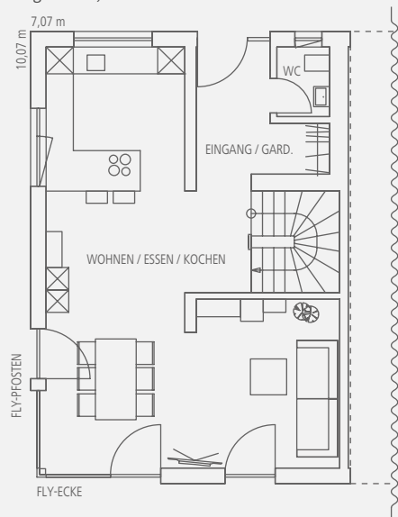
Erdgeschoss, ca. 58 m 2 NGF.
