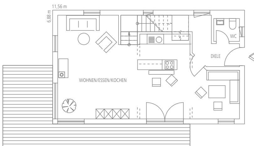
Erdgeschoss, ca. 66 m 2 WF.
