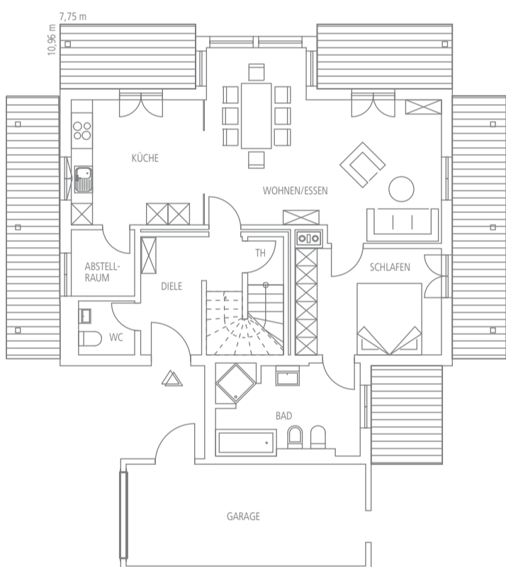
Erdgeschoss, ca. 84 m 2 WF.
